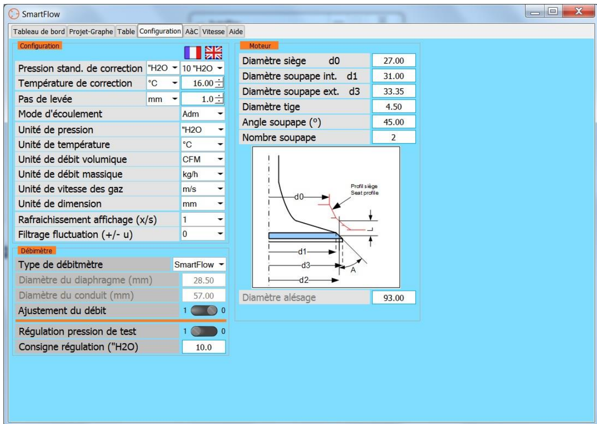
Figure 10 Ecran de configuration.
